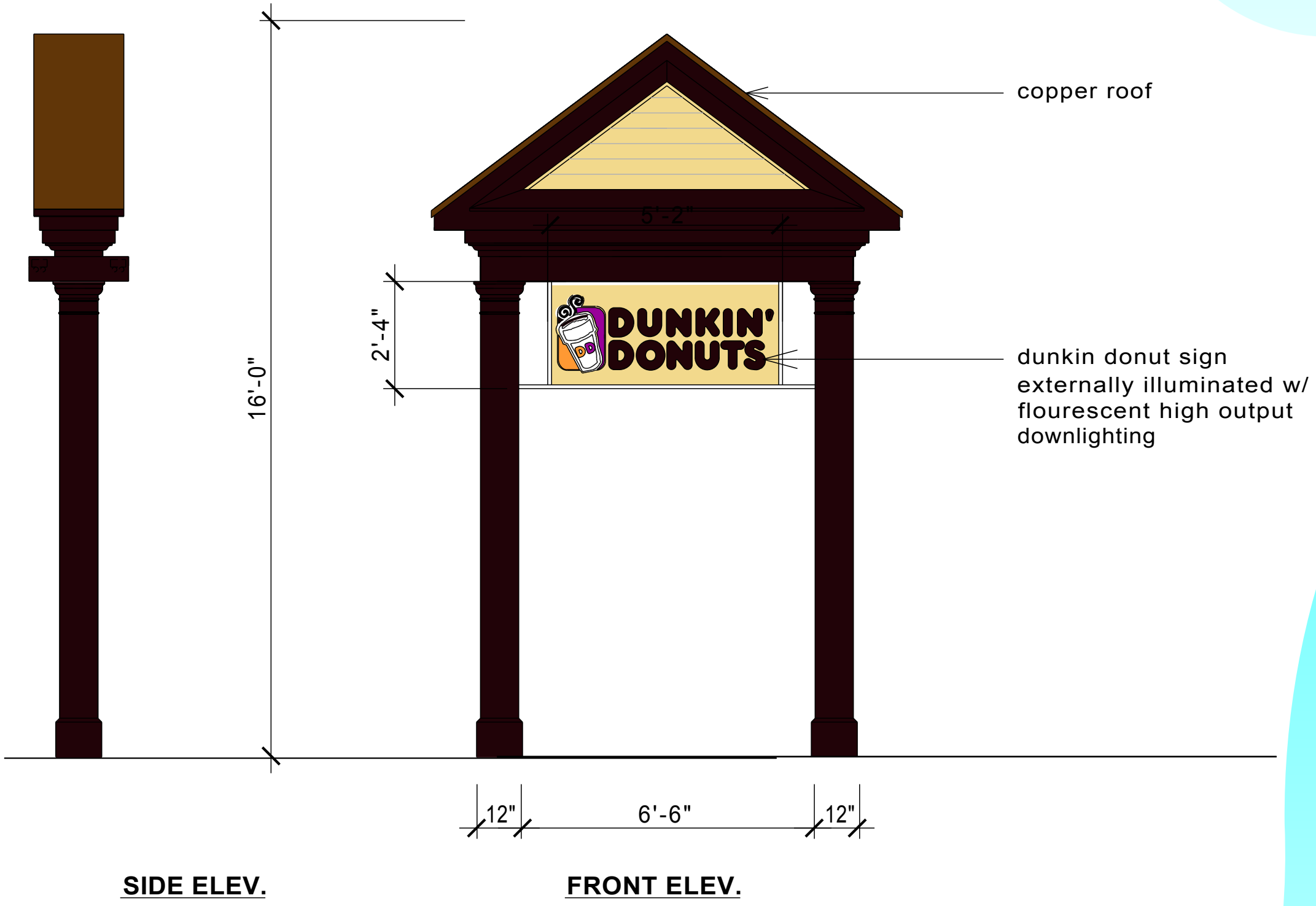
DD FREESTANDING PYLON SIGN
